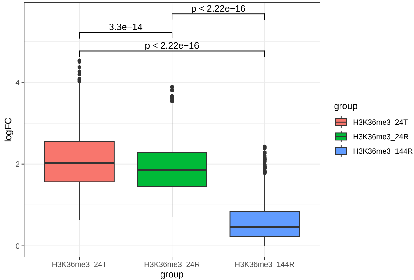
Absolute LFC across time for H3K36me3 set2
